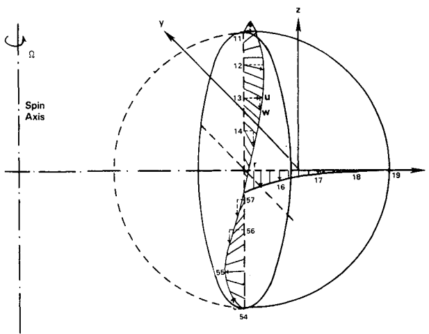
Fig. 4 First elevation slosh mode.
